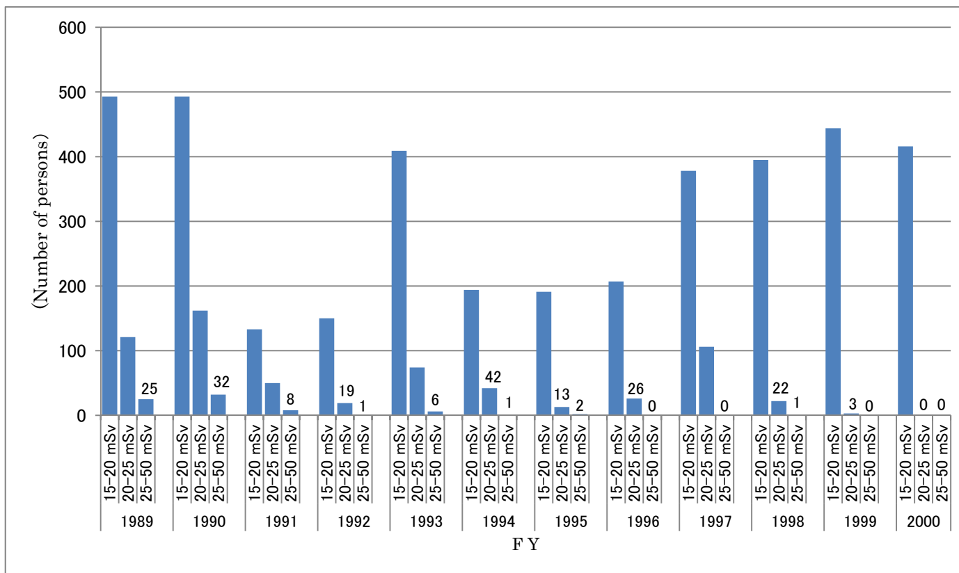
Number of Persons with Annual Dose Value Greater than 15 mSv of the NPPs in Japan(1989~2000)
